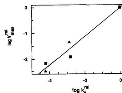
Figure 3. Hammett plot of \log V_{\text{max}}^{\text{rel}} versus \log k_p^{\text{rel}} for derivatives for 1 where Y = CH 3 , CH 2 F, and CHF 2 .
