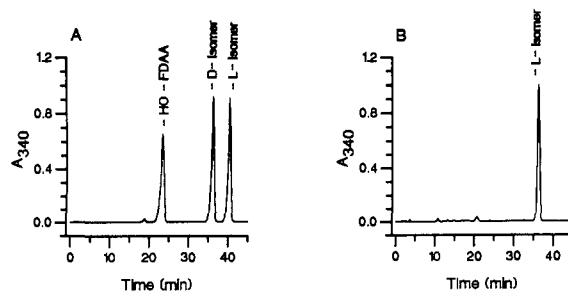
Figure 1. Chromatographic traces of FDAA-derivatized samples of 7-methyltryptophan (2-CH 3 ): (A) D,L mixture; (B) L-2-CH 3 isolated from acylase I hydrolysate of racemic 2-CH 3 .
