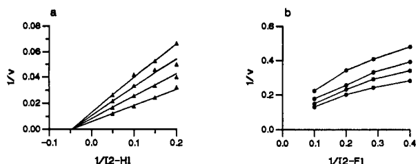
Figure 2. Double reciprocal kinetic plots for DMAT synthase: (a) varied 2-H at fixed concentrations of 1-CH 3 ,OPP; (b) varied 2-F at fixed concentrations of 1-CH 3 ,OPP.
