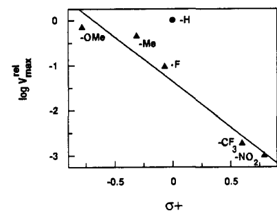
Figure 4. Hammett plot of \log V_{\text{max}}^{\text{rel}} versus \sigma^+ for derivatives of 2 where Z = H, OCH 3 , CH 3 , F, CF 3 , and NO 2 .
